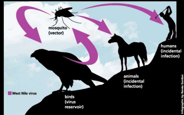
West Nile Virus Transmission Cycle
